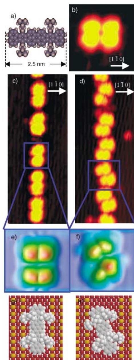
Figure 3. a) Filled-space model of the Violet Lander (VL) molecule; b) typical 3 \times 3 nm 2 STM image of the VL molecule on a clean Cu(110) surface, which reveals the VL as four lobes corresponding to the spacer legs (see text); c,d) 8 \times 20 nm 2 STM images showing the molecular chains formed after the deposition of VL on the nanopatterned O–Cu surface. The molecules adsorb exclusively on bare Cu stripes, but their orientation is no longer perpendicular to the direction of the chain. The molecules are found either perfectly aligned with the direction of the chain (c) or forming an angle of 20^\circ with respect to that direction (d); e,f) ESQC-simulated STM images of the VL on the bare Cu stripes, with two different adsorption geometries; g,h) ball models of the VL adsorbed on the nanopatterned Cu–O surface from which the simulated STM images e) and f) were extracted.
