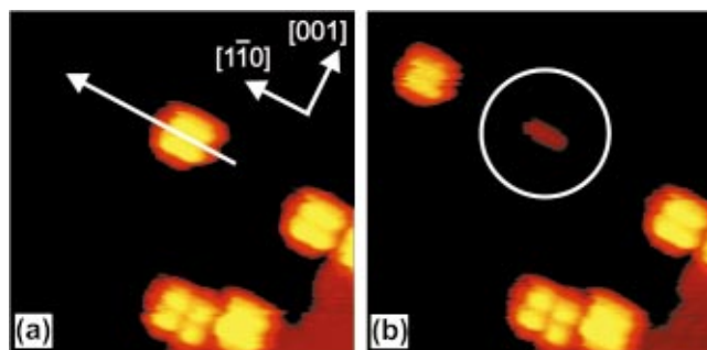
FIG. 5. (Color) Manipulation sequence of a Lander molecule on a Cu(110) terrace at 95 K after RT deposition ( 150 \times 150 \text{ \AA}^2 , V = -1769 \text{ mV} , I = -0.28 \text{ nA} ). (a) Before manipulation. The arrow marks the manipulation direction. (b) After manipulation (tunneling parameters for manipulation, V = -11 \text{ mV} , I = -3.1 \text{ nA} ). The circle marks the Cu rows that are visible where the molecule was adsorbed before.
