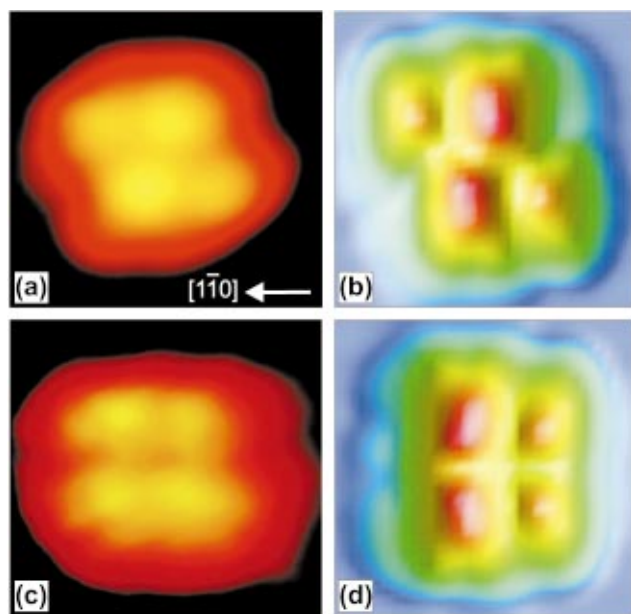
FIG. 2. (Color) STM image of a Lander molecule on Cu(110) at 100 K ( 20 \times 20 \text{ \AA}^2 , V = -1000 \text{ mV} , I = -0.21 \text{ nA} ) with (a) rhomboidal shape and (c) rectangular shape. (b) and (d) ESQC-calculated STM images of the rhomboidal (chiral) and rectangular (achiral) Lander molecules, respectively, using the same tunneling parameters as in the experiments. The aromatic board of the Lander molecules is parallel to the close-packed Cu direction indicated in the image.
