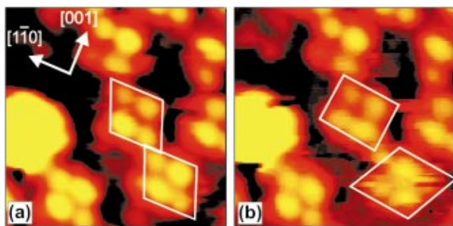
FIG. 3. (Color) STM images of Lander molecules revealing conformational changes ( 50 \times 50 \text{ \AA}^2 , V = -1000 \text{ mV} , I = -0.25 \text{ nA} ). (a) The center and lower-right molecule show the same rhomboidal shape. (b) The center molecule changed to the rectangular shape, while the lower-right molecule reveals a fluctuating conformation while imaging, with a dominating rhomboidal shape mirror symmetric to the original shape.
