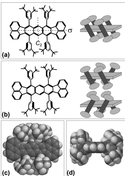
FIG. 1. Molecular structure of the Lander molecule ( C_{90}H_{98} ) consisting of a central polyaromatic board (terminated by two fluoranthene groups) and four spacer legs (3,5-di- tert -butylphenyl substituents). (a) Achiral form with C_{2h} symmetry: eclipsed conformation of legs on opposite sides of the board as better seen from the schematic drawing. The symmetry elements (rotation and mirror axes) are indicated. (b) Chiral form with C_2 symmetry: staggered conformation of legs on opposite sides of the board, which results in two enantiomers (indicated in the schematic drawing). The rotation axis runs perpendicular to the paper plane through the center of the molecule. Space-filling model of a chiral form: (c) top view and (d) side view (along the board) showing how the spacer legs separate the central board from the surface.
