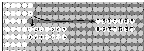
FIG. 6. Labelling of atoms in a nanostructure attached to a step (1–14) and on the terrace ( \bar{1} – \bar{14} ) referring to Table I. k marks a kink atom.
