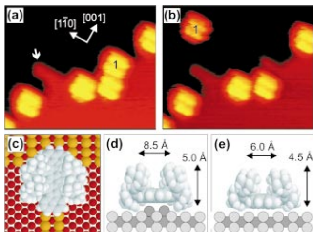
FIG. 4. (Color) (a) Before manipulating the Lander molecule labeled “1” from a Cu(110) step edge ( 136 \times 112 \text{ \AA}^2 , V = -1768 \text{ mV} , I = -0.37 \text{ nA} , T = 95 \text{ K} ). A nanostructure from a previous manipulation experiment is visible and indicated by an arrow. (b) After the manipulation of the molecule along the [1\bar{1}0] direction the nanostructure underneath becomes visible (tunneling parameters for manipulation; V = -55 \text{ mV} , I = -1.05 \text{ nA} ). (c) Model of the Lander on the nanostructure, showing that the board is parallel to the nanostructure. For clarity, the length of the nanostructure is extended beyond the molecule. Cross-sectional side view of the Lander (d) on a nanostructure and (e) on a flat terrace. The distance between and height of the spacer groups (from calculated STM images) are stated.
