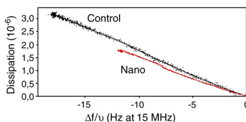
Fig. 6. \Delta D/\Delta f plot (at 15 MHz) of anti-IgG adsorbed on control and nanoporous titanium surfaces after initial adsorption of IgG.
