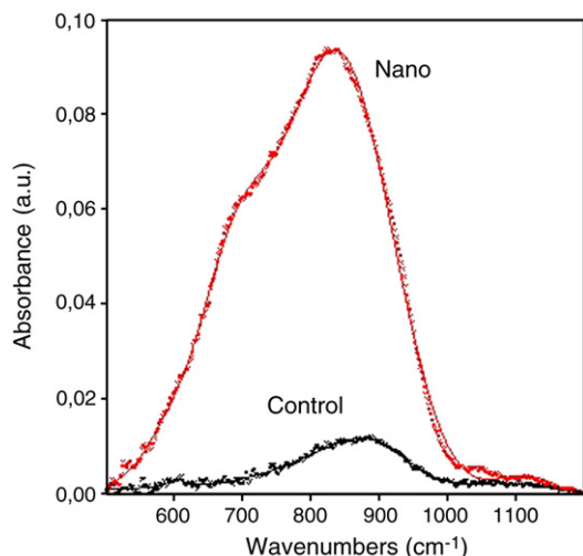
Fig. 2. FTIR spectra of sputtered titanium before (Control) and after (Nano) treatment with H_2SO_4/H_2O_2 .
