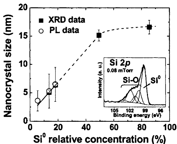
FIG. 3. Si nanocrystal size calculated from XRD and PL data as a function of the ratio “nonoxidized Si/total Si” obtained by XPS analysis in as-deposited films. In the inset, an example of Si 2 p peak deconvolution onto nonoxidized (Si 0 ) and oxidized (Si–O) components (sample deposited under 0.08 mTorr).
