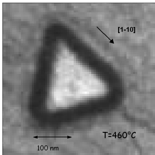
FIG. 4. 500 \times 500\text{-nm}^2 LEEM image of a typical triangular island acquired from a sample grown at 460^\circ\text{C} . Note that the regular structure of the facets that bound the island does not seem to be affected by the steps visible on the WL.
