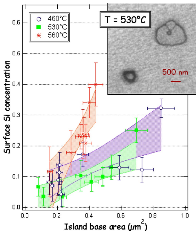
FIG. 6. (Color online) Silicon surface concentration for selected islands vs their basal areas plotted with 90% confidence bands. Islands were grown at the indicated temperatures. Note that the 460 and 530^\circ\text{C} confidence bands overlap over the entire accessed range. Inset: 4.5 \times 4.5\text{-}\mu\text{m}^2 LEEM image of a sample grown at 530^\circ\text{C} . Ripened atoll-like structures coexist with smaller islands.
