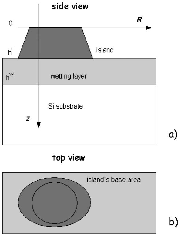
FIG. 1. Schematic representation of a portion of the sample with a modeled island: (a) side view and (b) top view.
