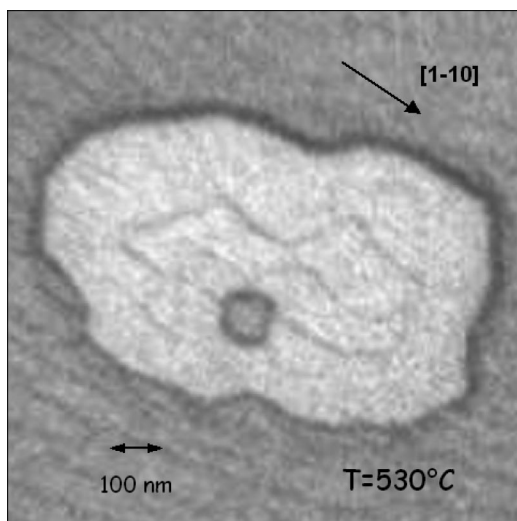
FIG. 5. 1 \times 1\text{-}\mu\text{m}^2 LEEM image displaying an example of the largest observed islands, from a sample grown at 530^\circ\text{C} . The atoll-like morphology is clearly visible with an asymmetric depletion that seems to expose an inner portion of the WL.
