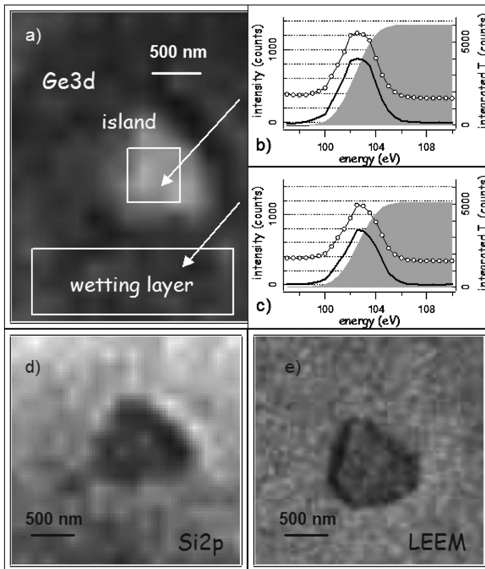
FIG. 2. (a): 2.5 \times 3.4\text{-}\mu\text{m}^2 XPEEM image, integrated over the \text{Ge}3d photoelectron kinetic energies, displaying the typical island-wetting layer \text{Ge}3d contrast; (b) and (c): \text{Ge}3d photoelectron spectra, averaged over the regions labeled in (a): (b) from the top base of the 3D island, (c) from the wetting layer: circles: raw data; thick line: background-subtracted data; shadowed curve: overall intensity, used in the equations; (d): 2.8 \times 2.8\text{-}\mu\text{m}^2 XPEEM image over the \text{Si}2p photoelectrons peak, displaying the same island shown in (a) as a dark structure on the bright wetting layer; and (e): 2.8 \times 2.8\text{-}\mu\text{m}^2 LEEM image of the island in (a), showing its faceted structure. The deposition temperature was 530\text{ }^\circ\text{C} .
